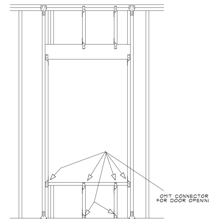
WINDOW AND DOOR OPENING CONNECTION DETAIL CONSULT CONNECTION MANUFACTURER FOR SPECIFIC CONNECTOR NAME
