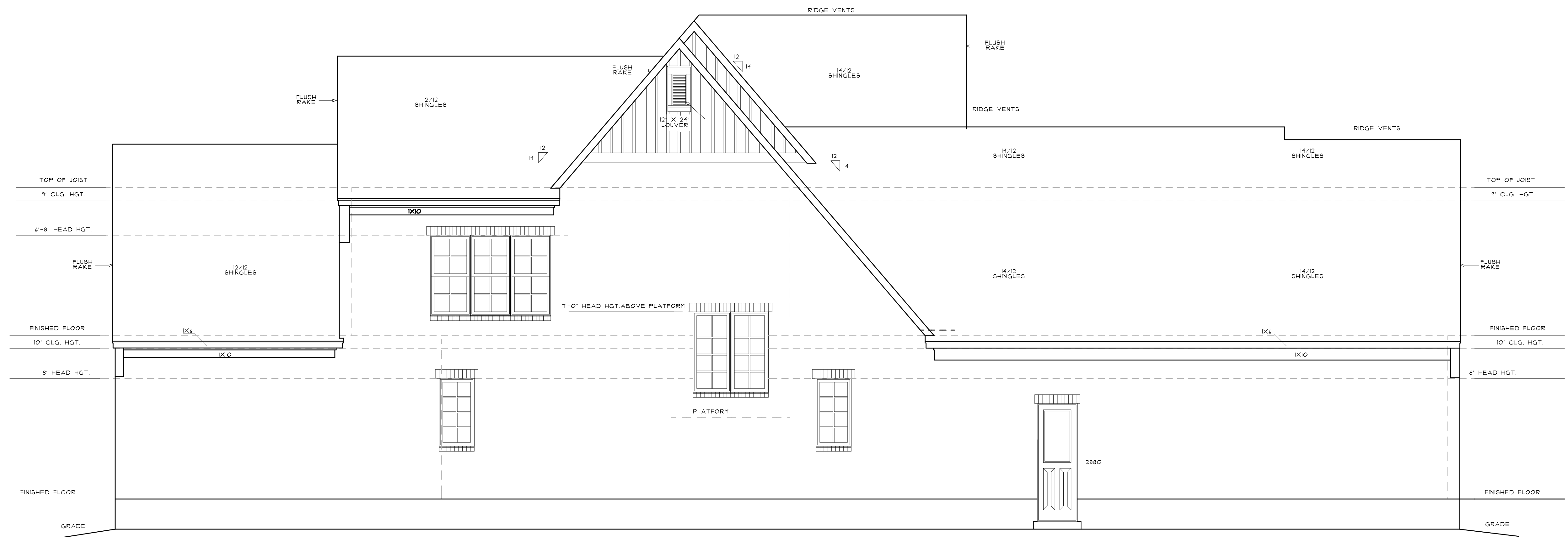
LEFT ELEVATION
