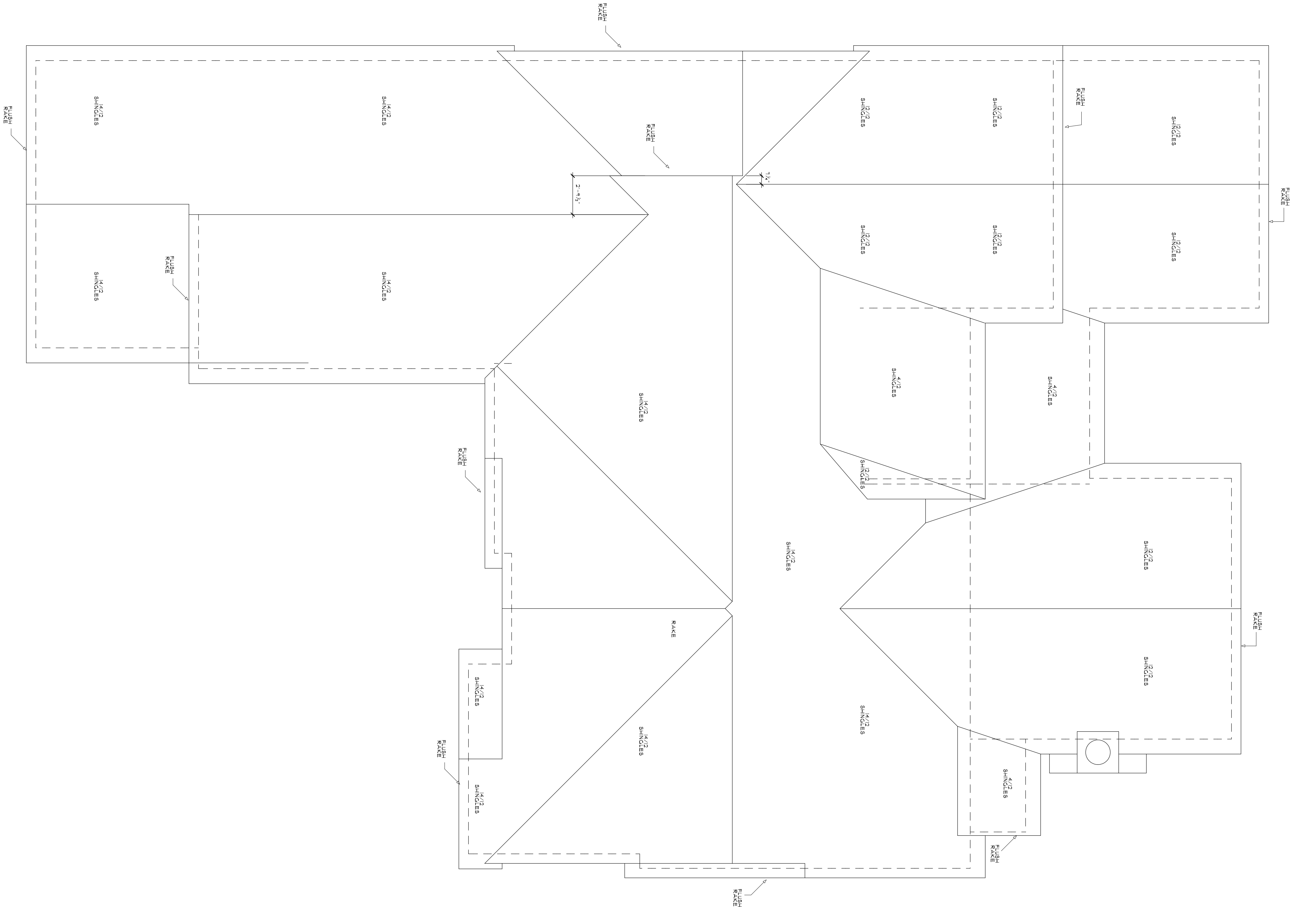
ROOF PLAN
