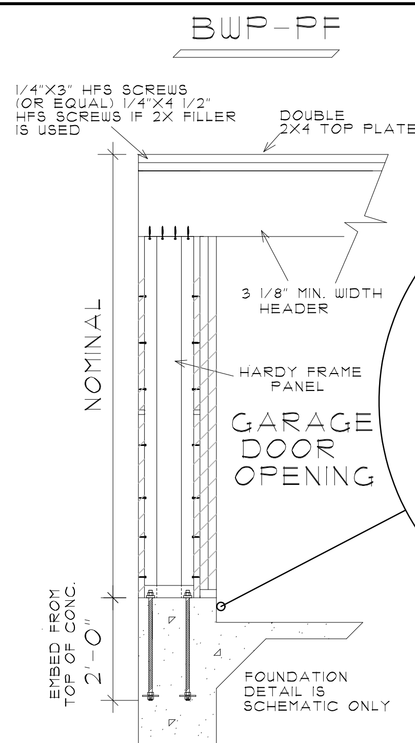
HARDY FRAME PANEL GARAGE FRONT
