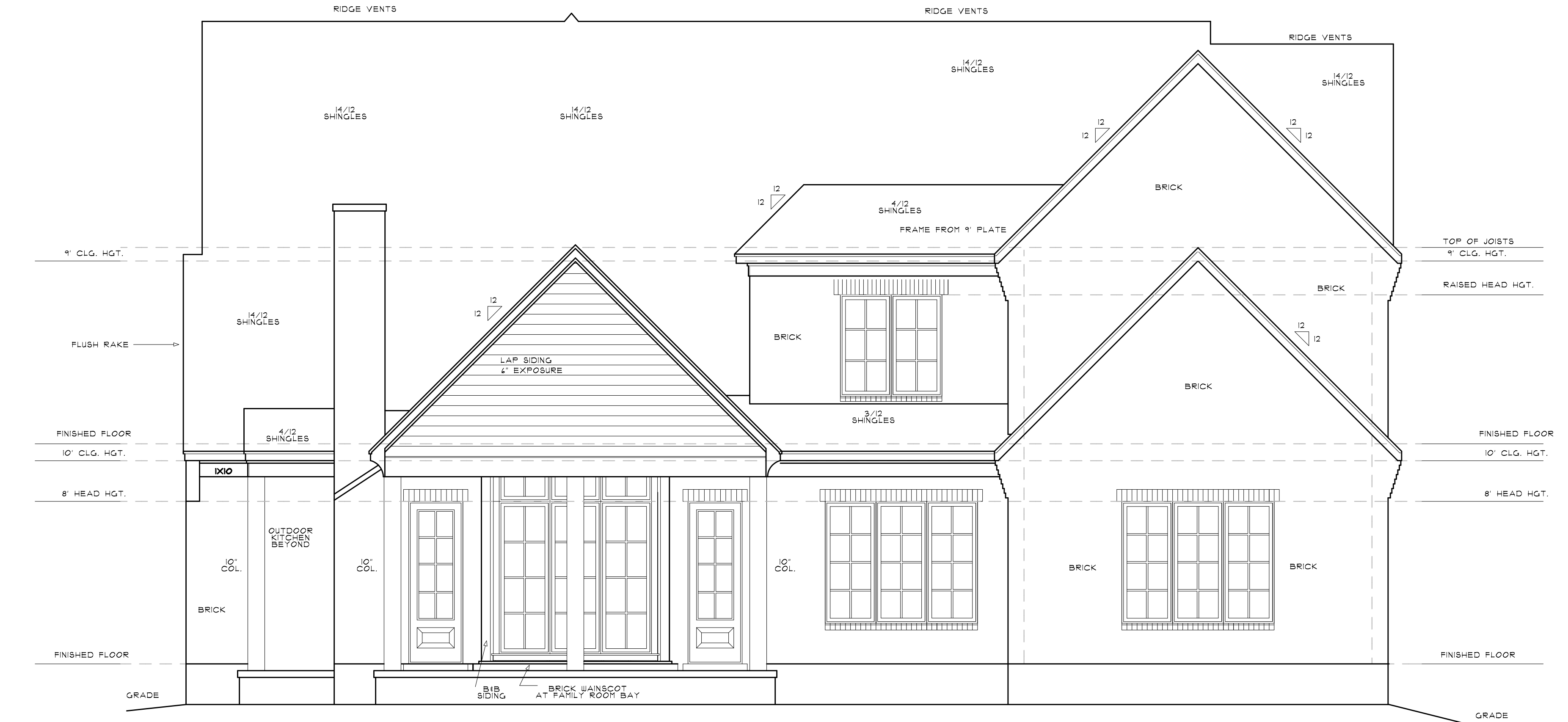
REAR ELEVATION
