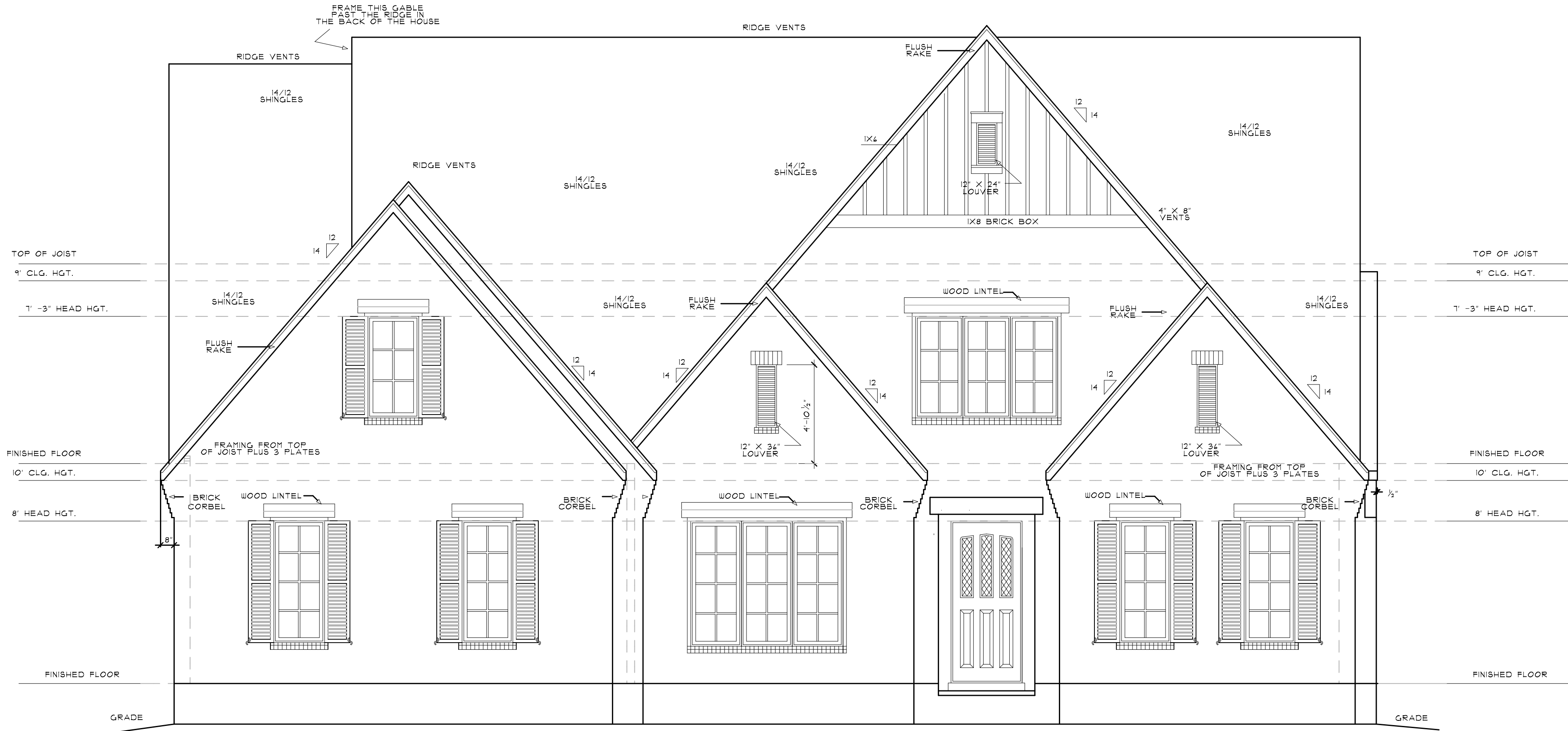
FRONT ELEVATION
